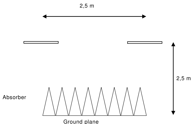
Figure 19 – Set-up for LPDA antennas above absorber
