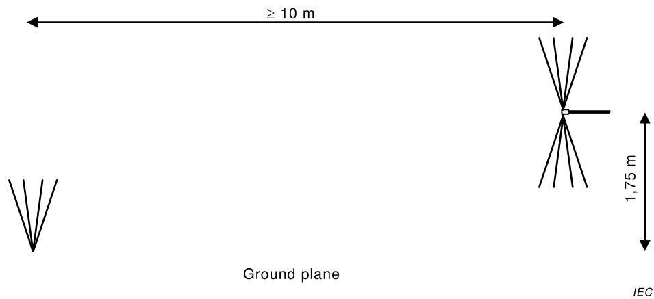
Figure 17 – Biconical antenna set-up for SAM using vertical polarization, showing the paired monocone antenna and an example collapsible-element biconical AUC
