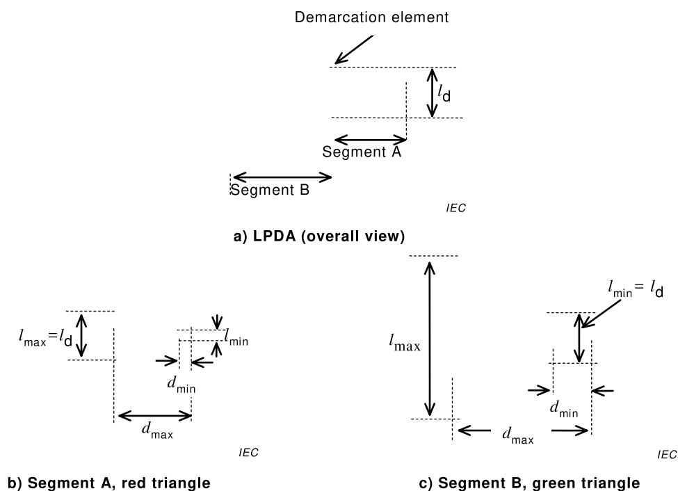
Figure 14 – LPDA antenna with a tapered curved geometry
